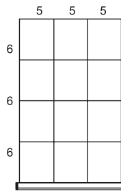
L_BG-A0209 12 compartments
