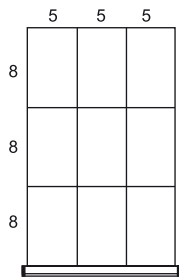
L_BG-A0206 9 compartments
